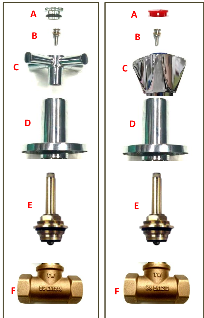
Exploded View
